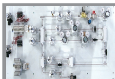
高压管路系统 High-pressure Duct System
