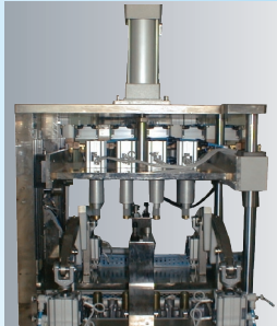
火花塞封堵自动提升装置 Spark plug plugging auto lifting device
